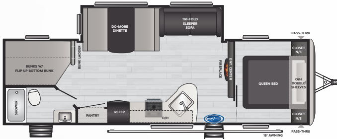
282BHWE | WEIGHT 6621 | LENGTH 32' 2"
