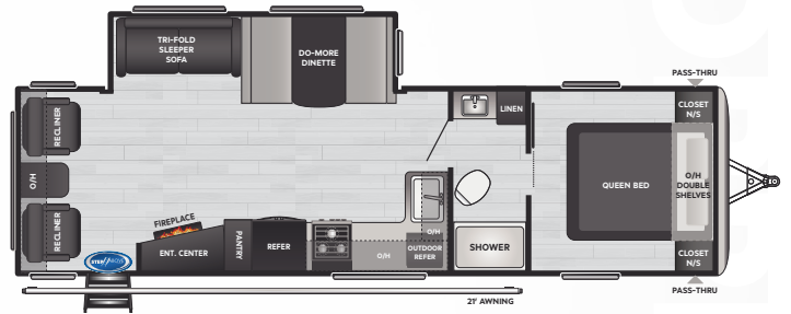
285TLWE | WEIGHT 6748 | LENGTH 33' 6"
