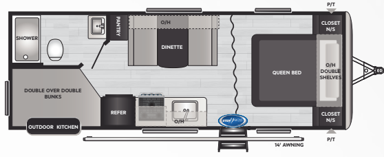
220BHWE | WEIGHT 4880 | LENGTH 26' 11"
