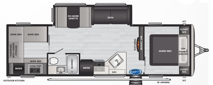
298BHWE | WEIGHT 6705 | LENGTH 32' 9"
