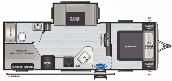
240BHWE | WEIGHT 5915 | LENGTH 28' 11"
